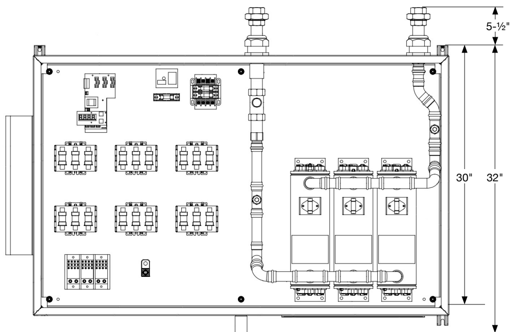
FRONT VIEW
